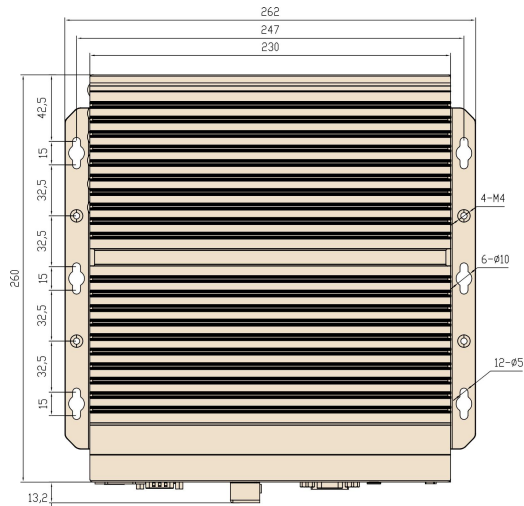
RIRR-IPC-BOX-H420-A2-260 机身长度260mm
